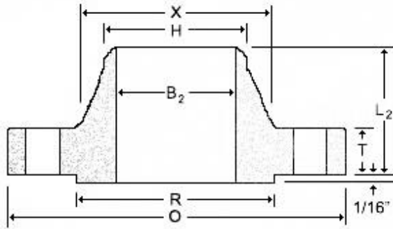
ANSI B16.47 SERIES B CLASS 75 FLANGES DIMENSIONS TABLE
