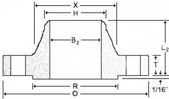
ANSI B16.47 SERIES A CLASS 150 FLANGES DIMENSIONS TABLE
