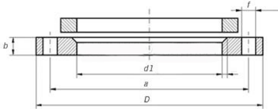
GERMANY STANDARD FLANGE DIN 2642 FOR WELDING PN 10
