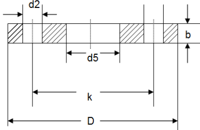
GERMANY STANDARD FLANGE DIN 2503 FOR SOLDERING OR WELDING PN 40
