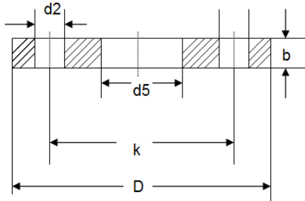
GERMANY STANDARD FLANGE DIN 2501 FOR SOLDERING OR WELDING PN 10
